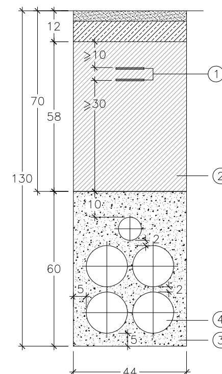
4\phi 160 + 1\phi 90 E=1/15
