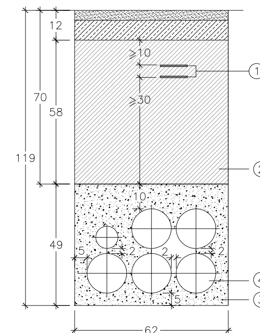
5\phi 160 + 1\phi 90 E=1/15
