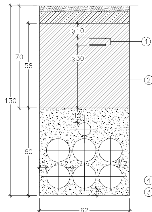
6\phi 160 + 1\phi 90 E=1/15
