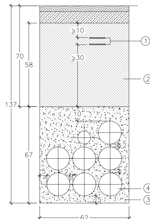
7\phi 160 + 1\phi 90 E=1/15
