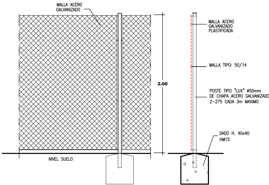
—DETALLE— —VALLADO TIPO—ARGA— Escala 1/40
