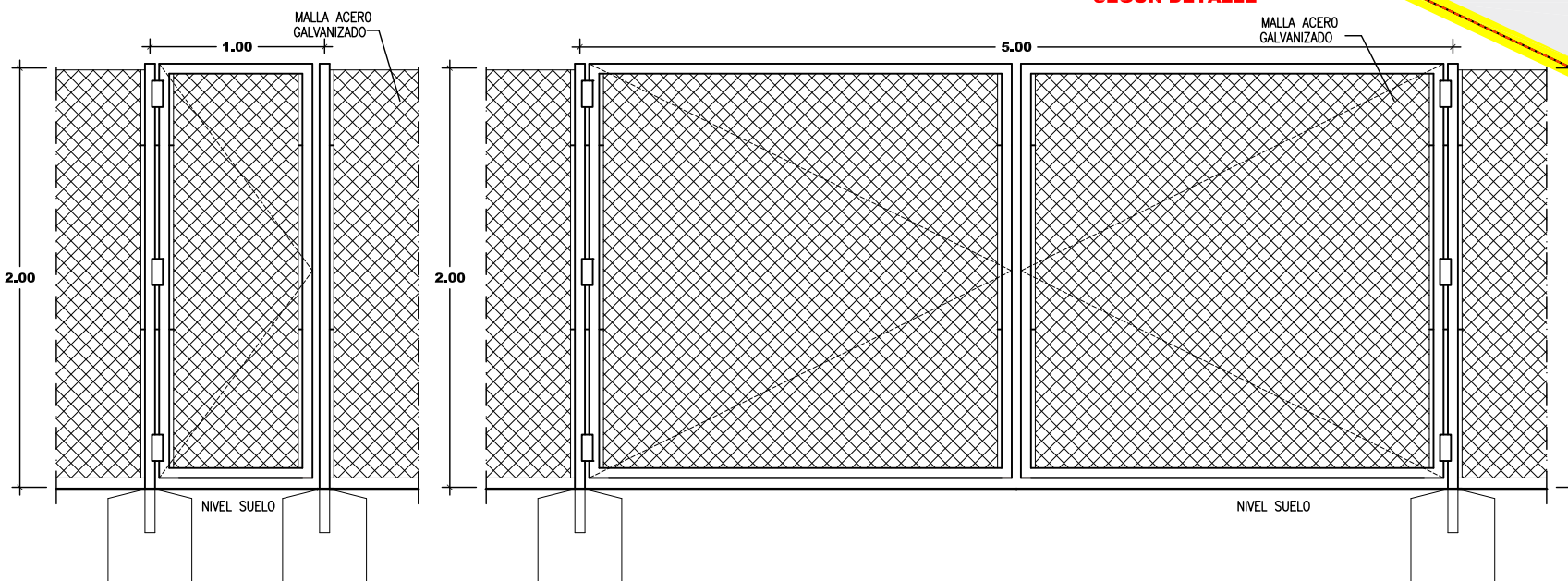
—DETALLE— —PUERTA TIPO—ARGA— Escala 1/40
